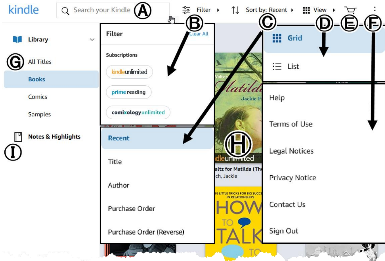
Figure 9 1: The Kindle cloud reader - library mode.
