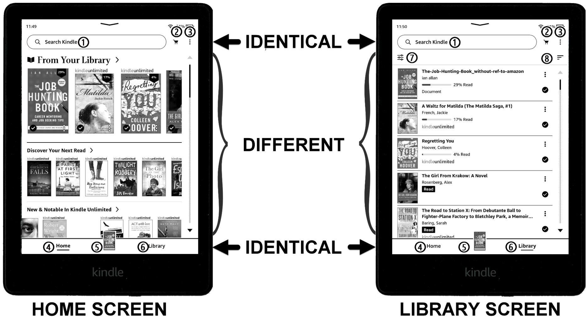
Figure 4-1: The Home screen and Library screen. The labels are described below.
